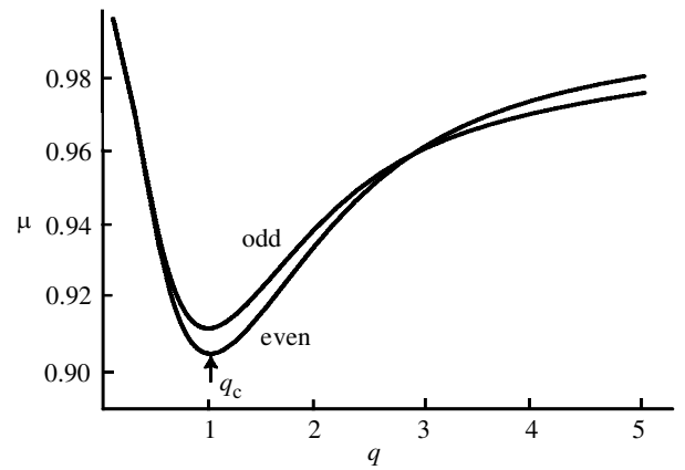
Figure 17. Same as figure 16 except that \hat{W}(q) satisfies equation (36) with \theta_0 = \pi/3 rather than equation (34). It can be seen that the marginally stable eigenmodes are now even functions of \phi .
