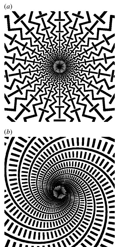
Figure 34. Action of the double inverse retinocortical map on odd rhombic planforms: (a) rhombic, (b) roll.
