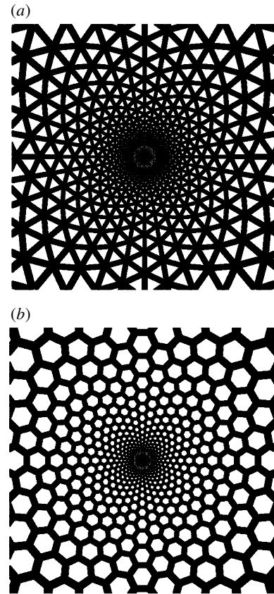
Figure 35. Action of the double inverse retinocortical map on even hexagonal planforms: (a) \pi -hexagonal, (b) 0-hexagonal.
