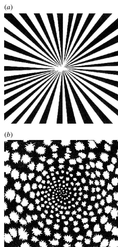
Figure 3. (a) Funnel and (b) spiral tunnel hallucinations generated by LSD. Redrawn from Siegel (1977).
