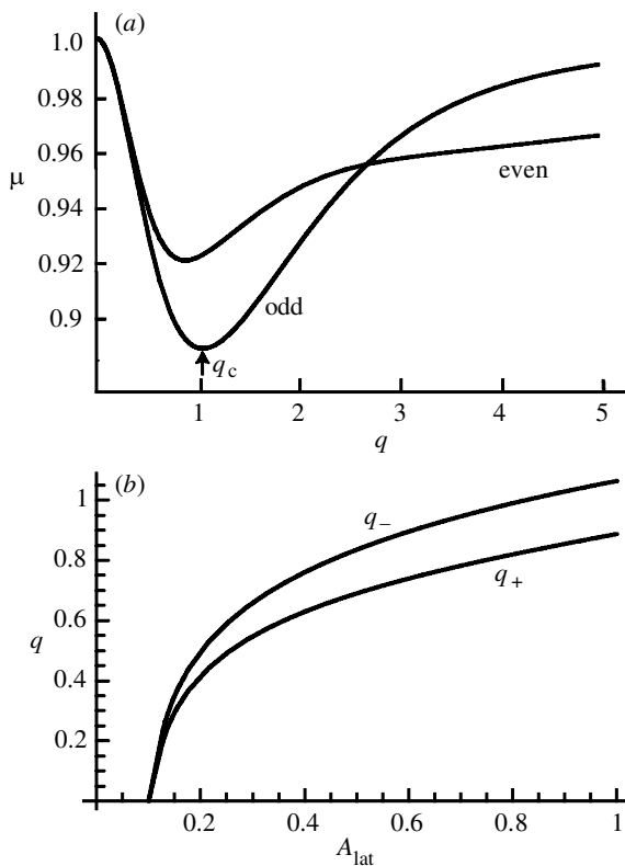
Figure 16. (a) Plot of marginal stability curves \mu_{\pm}(q) for g(s) given by the difference of Gaussians (equation (6)) with \xi_{\text{lat}} = 1 , \hat{\xi}_{\text{lat}} = 3 , A_{\text{lat}} = 1 and \beta = 0.4W_1 . Also set \alpha/\sigma_1 W_1 = 1 . The critical wavenumber for spontaneous pattern formation is q_c . The marginally stable eigenmodes are odd functions of \phi . (b) Plot of critical wavenumber q_{\pm} for marginal stability of even (+) and odd (−) patterns as a function of the strength of inhibitory coupling A_{\text{lat}} . If the inhibition is too weak then there is a bulk instability with respect to the spatial domain.
