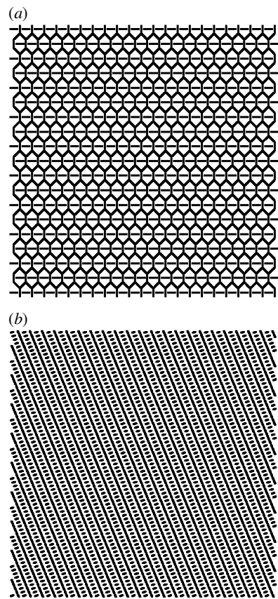
Figure 23. Contours of even axial eigenfunctions on the rhombic lattice: (a) rhombic, (b) roll.
