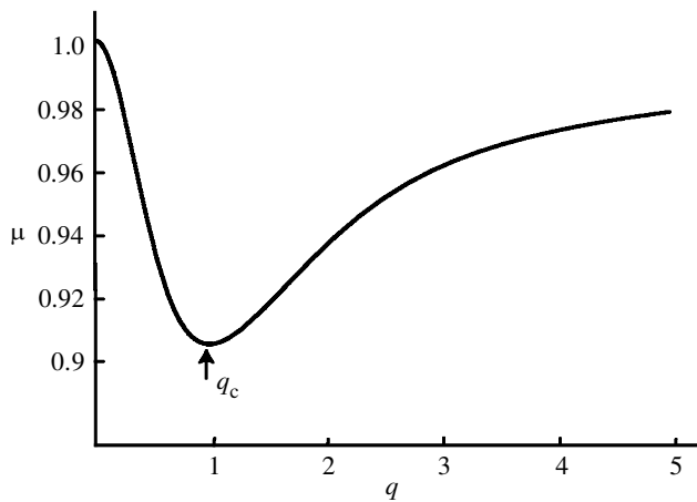
Figure 18. Plot of marginal stability curve \mu_0(q) for a bulk instability with respect to orientation and g(s) given by the difference of Gaussians (equation (6)) with \xi_{\text{lat}} = 1 , \hat{\xi}_{\text{lat}} = 3 , A_{\text{lat}} = 1.0 , \beta = 0.4W_0 and \alpha/\sigma_1 W_0 = 1 . The critical wave-number for spontaneous pattern formation is q_c .
