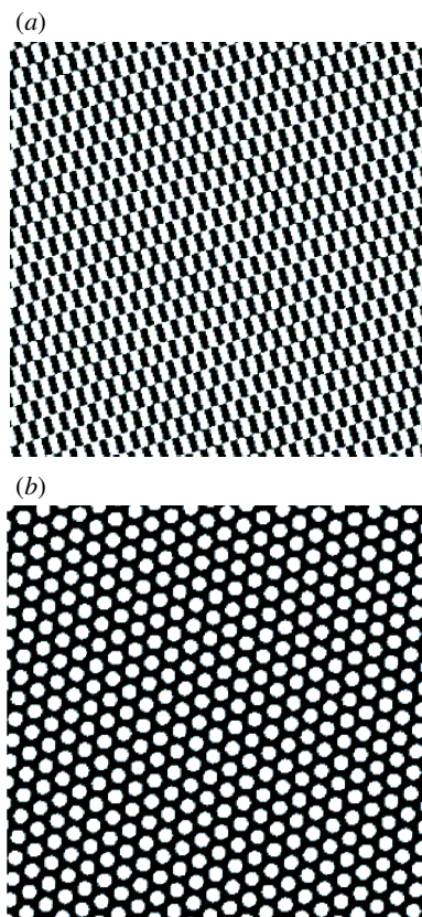
Figure 20. Non-contoured axial eigenfunctions on rhombic and hexagonal lattices: (a) rhombic, (b) hexagonal.
