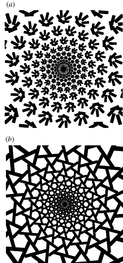
Figure 36. Action of the double inverse retinocortical map on odd hexagonal planforms: (a) triangular, (b) 0-hexagonal.
