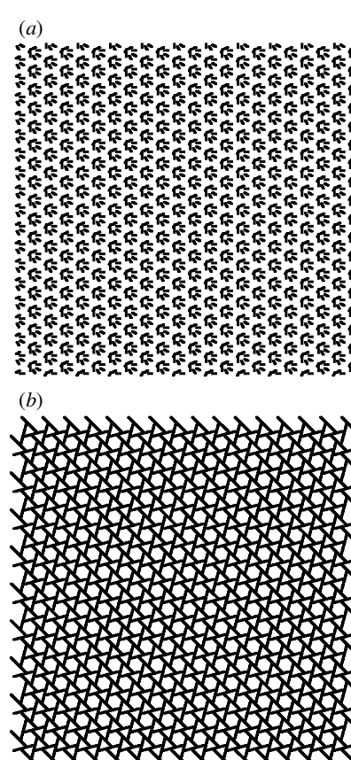
Figure 26. Contours of odd axial eigenfunctions on the hexagonal lattice: (a) triangular, (b) 0-hexagonal.
