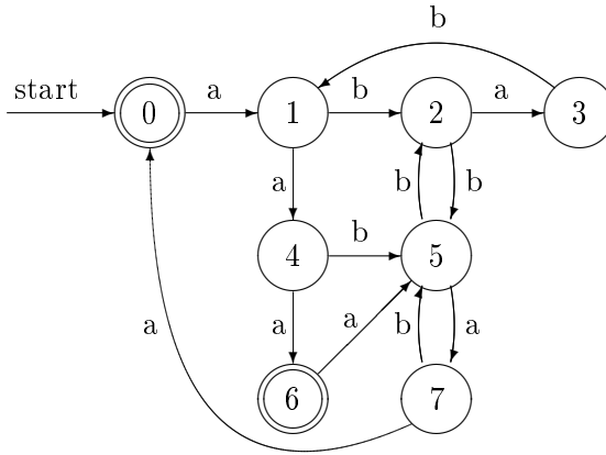
Figure 2.9: Non-minimal DFA
