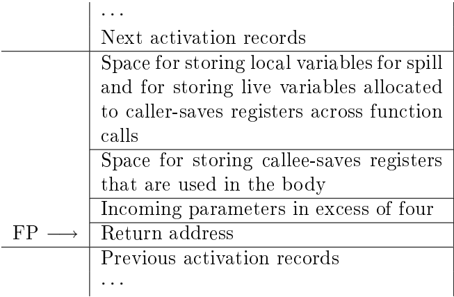
Figure 9.8: Activation record layout for the register division shown in figure 9.7
