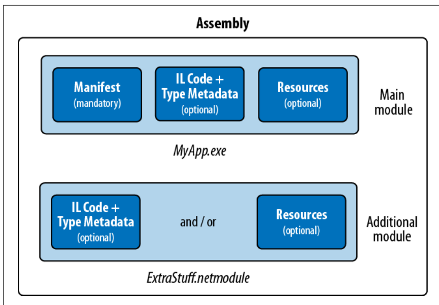
Figure 18-2. Multifile assembly
