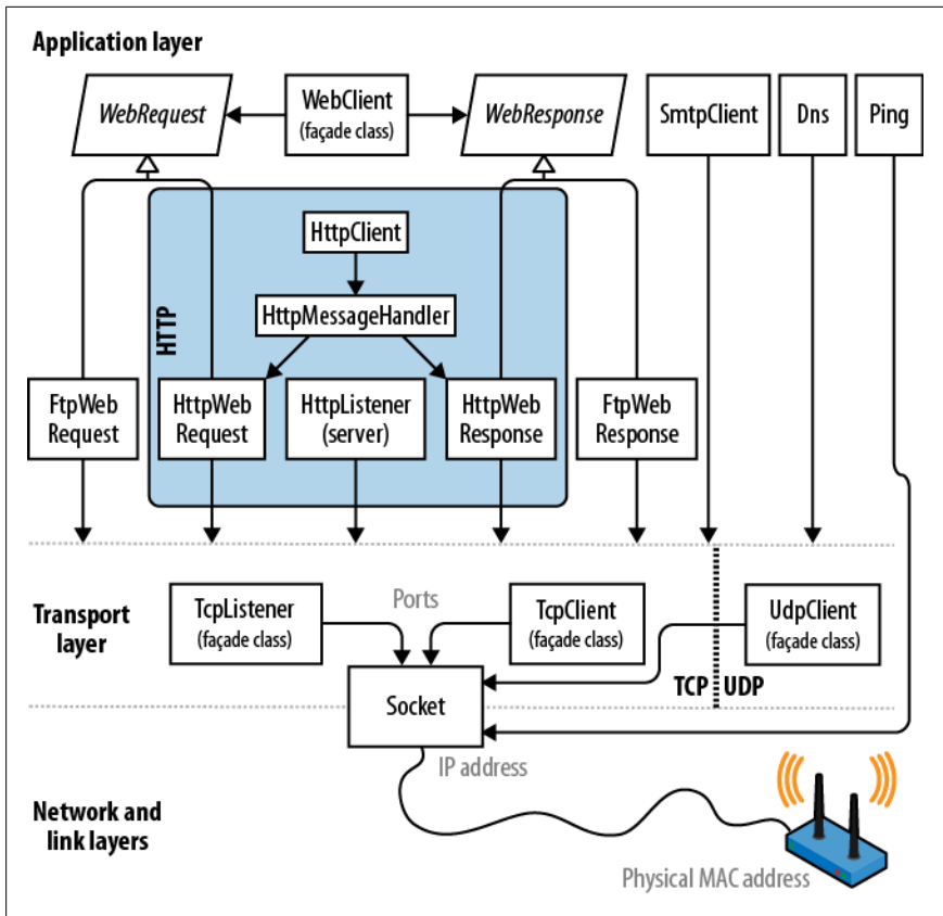
Figure 16-1. Network architecture
