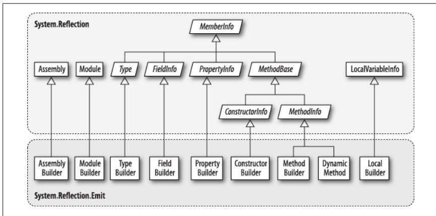
Figure 19-2. System.Reflection.Emit
