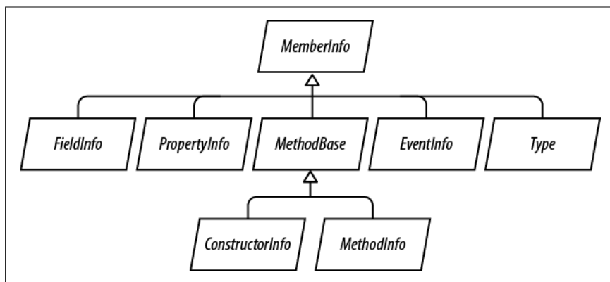
Figure 19-1. Member types
