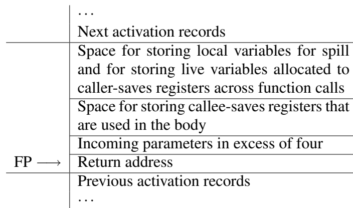
Figure 9.8: Activation record layout for the register division shown in figure 9.7
