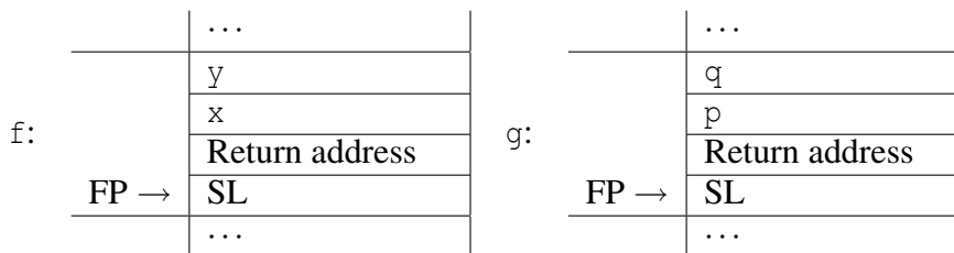
Figure 9.14: Activation records for f and g from figure 9.11
