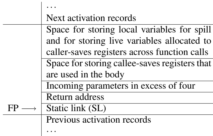
Figure 9.13: Activation record with static link
